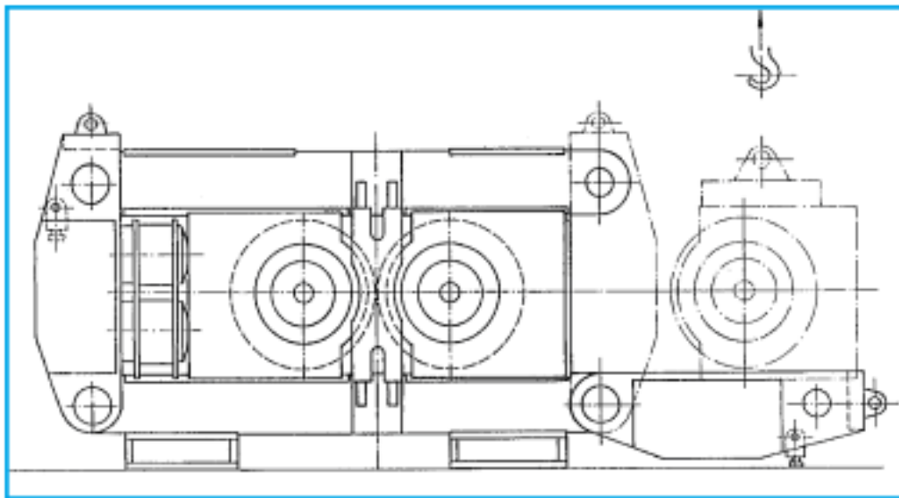
Fig. 3 Hinged Frame Design Klapprahmen
