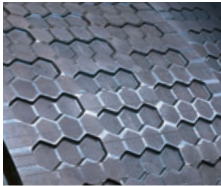
HEXADUR® standard surface and electrochemically machined, preconditioned surface
