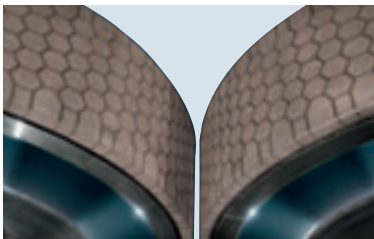
Rolls with HEXADUR® tires – view inside the working gap.
